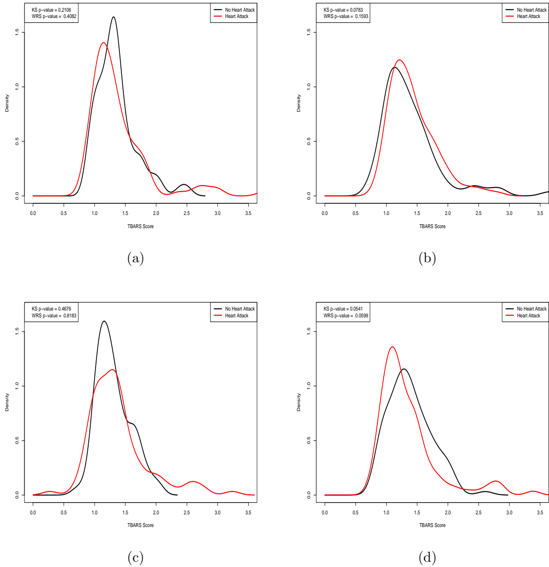
Figure 7: TBARS examples where the density-based EL distribution equality statistic is significant ( p value < 0.05 ), but the two-sample Kolmogorov-Smirnov (KS) test and two-sample Wilcoxon rank sum (WRS) test are not significant ( p values > 0.05 ).
